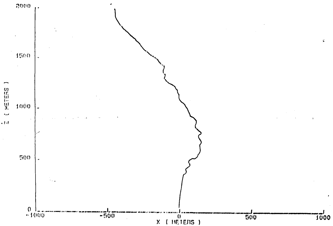
FIGURE 1. Computer reconstructed X-Z projection of a triggered lightning stroke. The straight channel from the ground is typical of "classical" triggering when the copper wire attached to the rocket is also electrically attached to the ground. The torturous path of the lightning channel higher up is typical of natural lightning.
